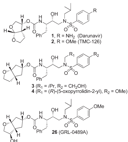
Figure 1. Structures of potent HIV-1 protease inhibitors 1–4 and 26.
